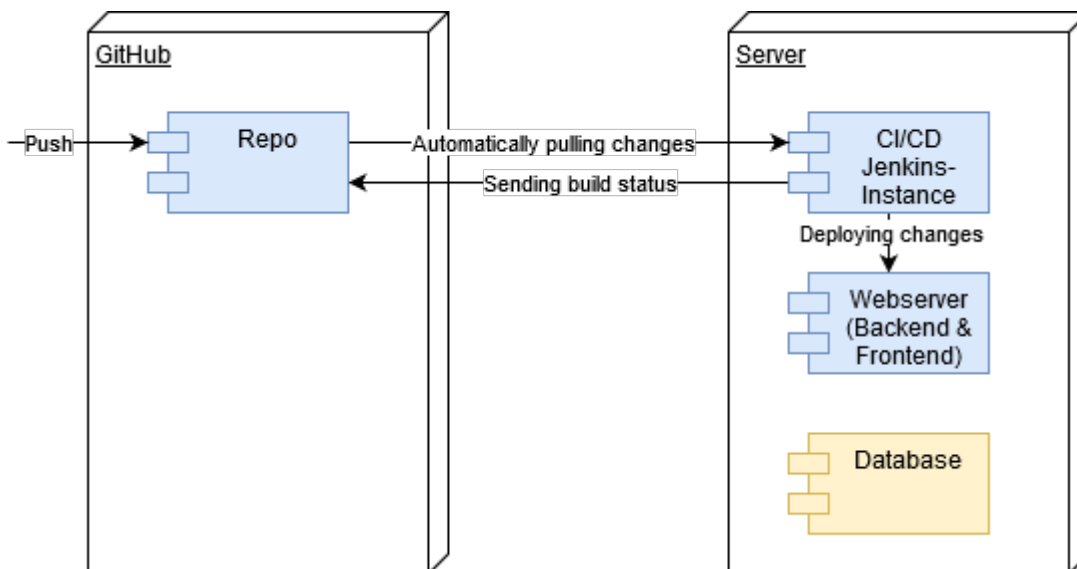
Deployment View
